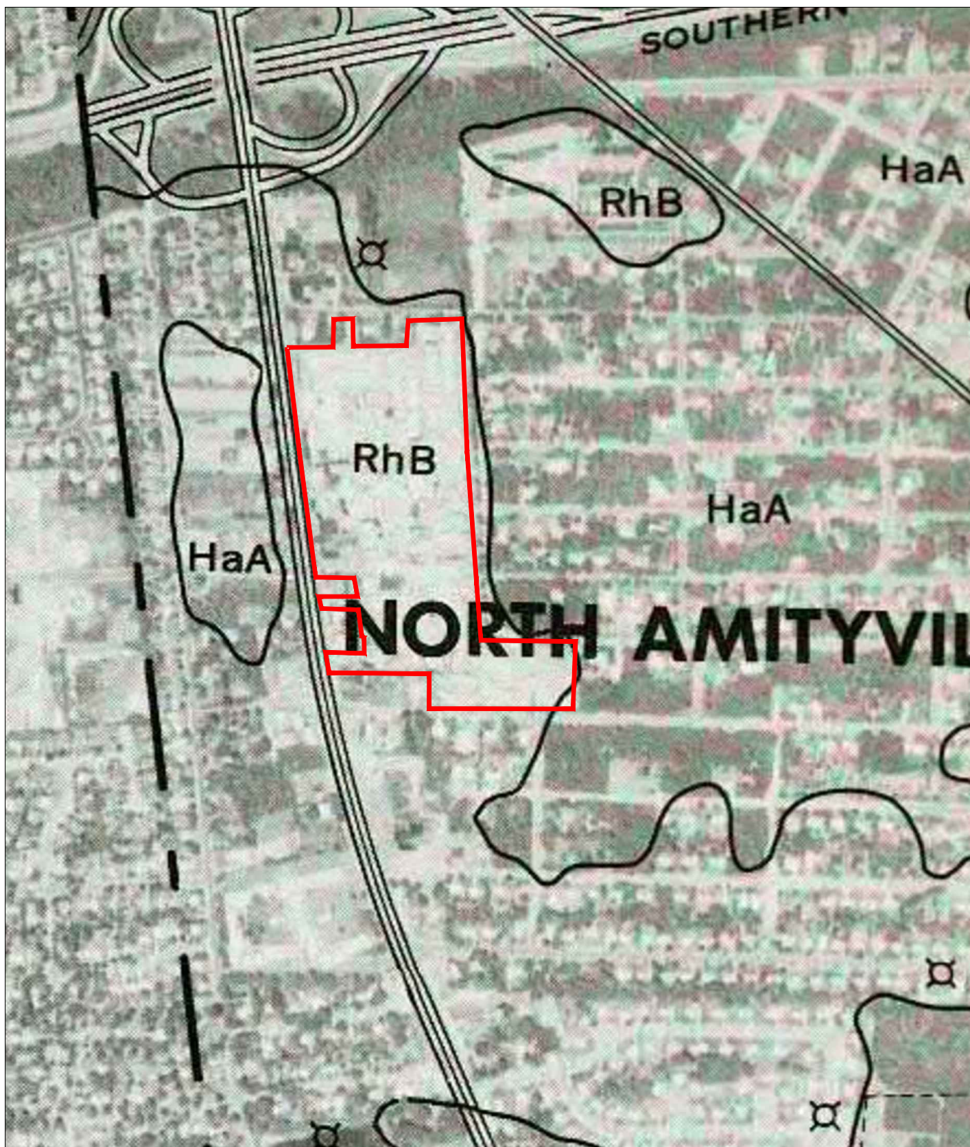
FIGURE 2-2 SOIL MAP
